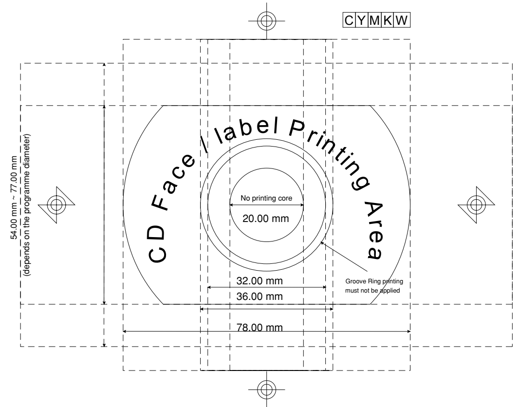
Cut 80.00 mm (Mini-Disk) ROM Offset print specifications
