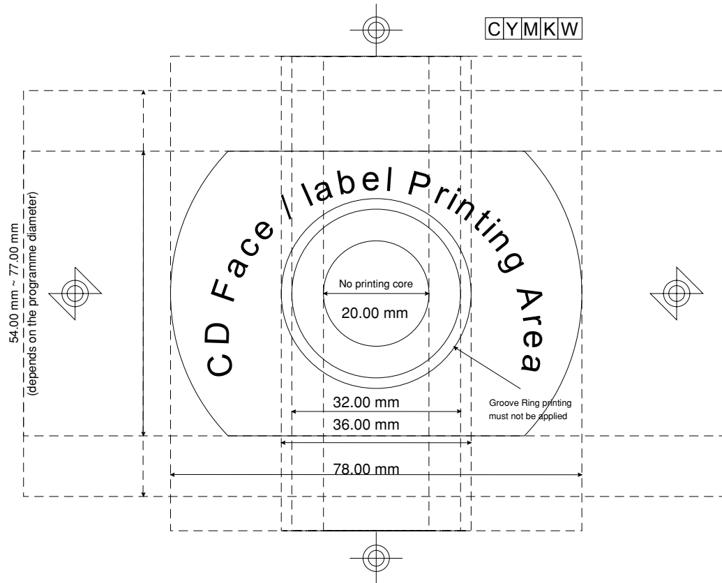
Cut 80.00 mm (Mini-Disk) ROM Screen print specifications
