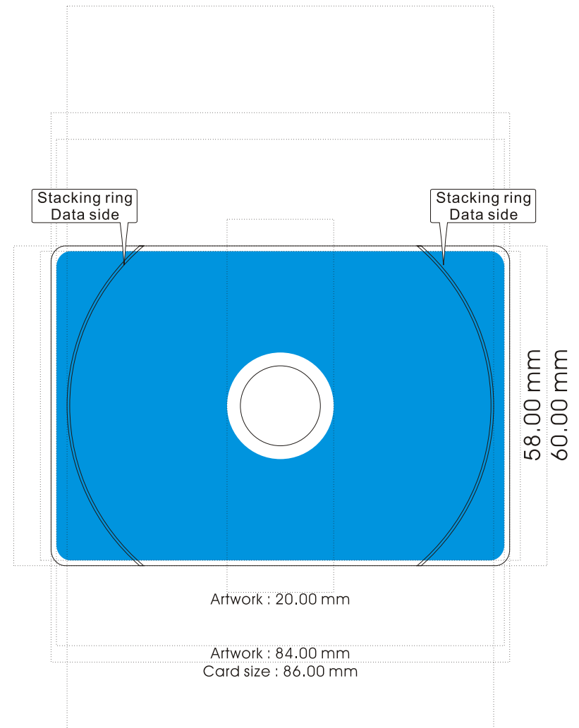
Stacking ring : 80.00 mm 60.00 mm X 86.00 mm Moulded Card CD without groove ring
