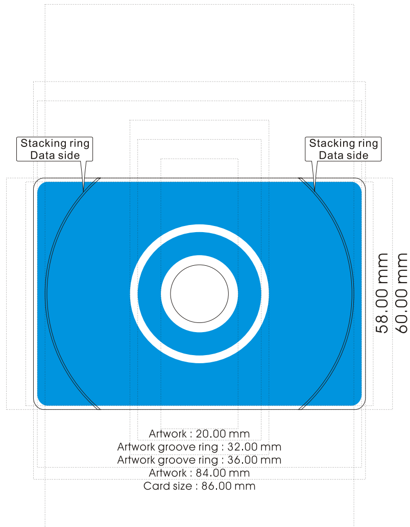
Stacking ring : 80.00 mm 60.00 mm X 86.00 mm Moulded Card CD with groove ring
